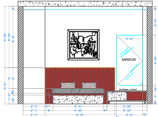
ELEVATION B EXTERNAL LAYOUT
