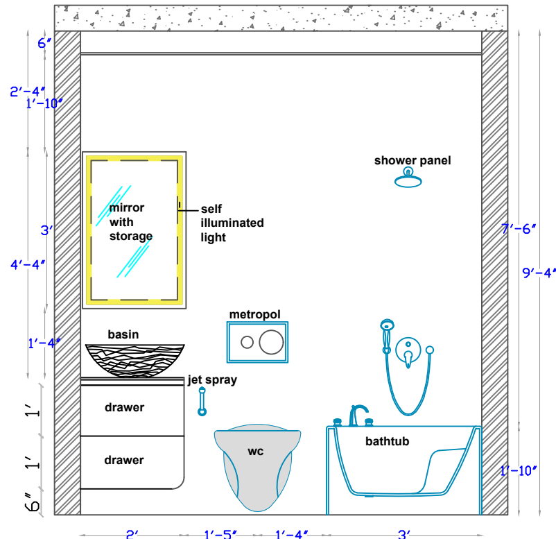
ELEVATION A EXTERNAL LAYOUT
