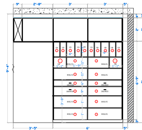
ELEVATION B INTERNAL LAYOUT
