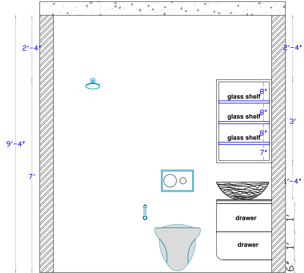
ELEVATION A INTERNAL LAYOUT
