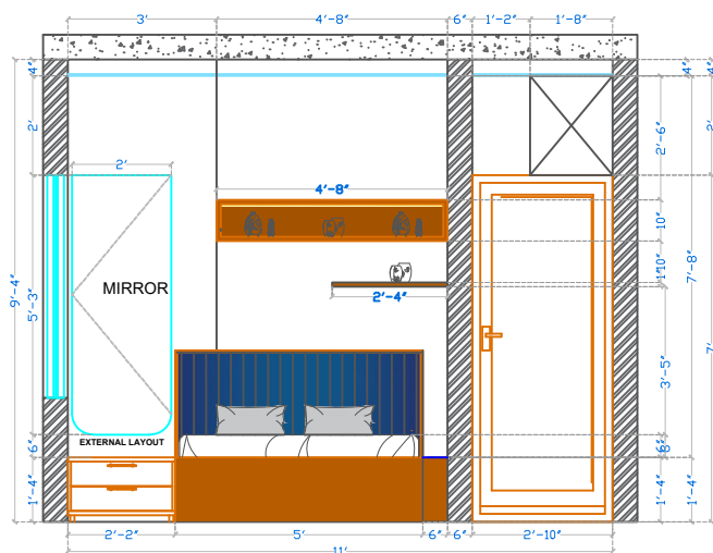
ELEVATION A EXTERNAL LAYOUT
