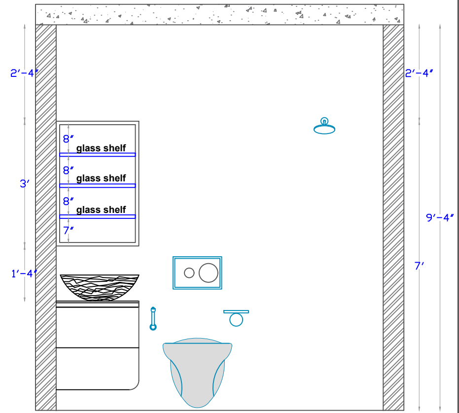
ELEVATION B INTERNAL LAYOUT
