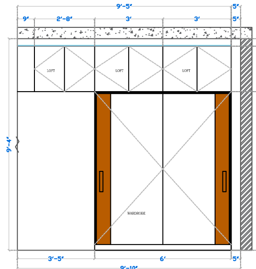
ELEVATION B EXTERNAL LAYOUT
