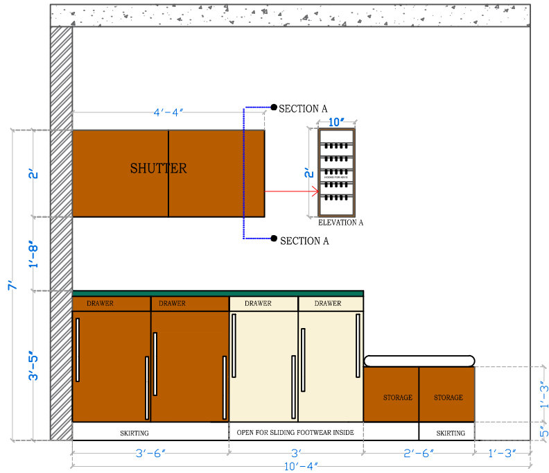
ELEVATION A EXTERNAL LAYOUT
