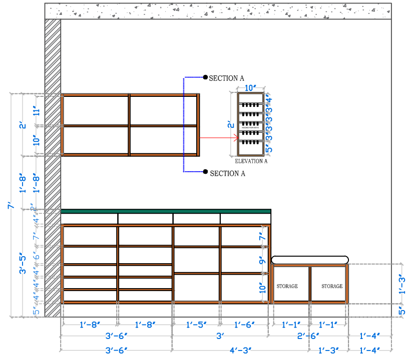
ELEVATION A INTERNAL LAYOUT
