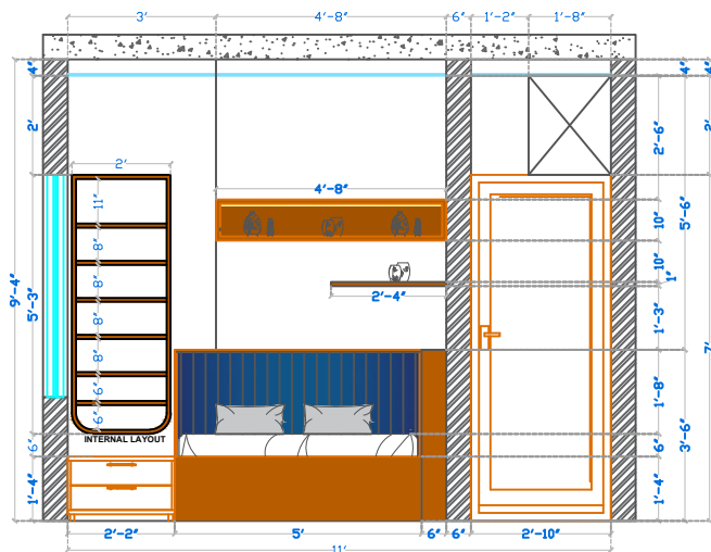
ELEVATION A INTERNAL LAYOUT
