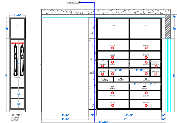
ELEVATION C INTERNAL LAYOUT
