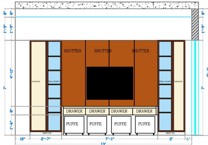
ELEVATION A EXTERNAL LAYOUT
