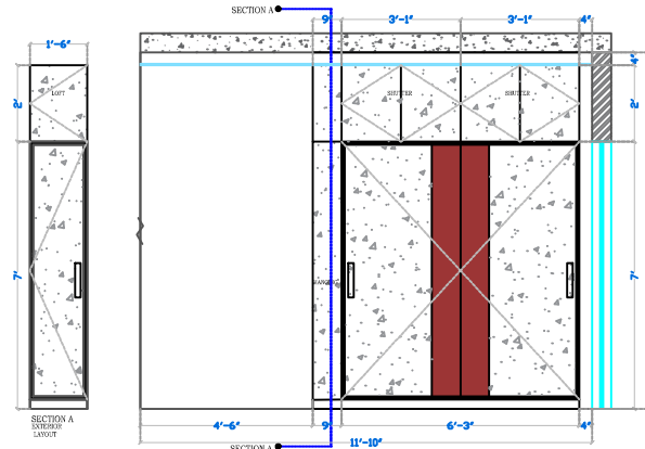
ELEVATION C EXTERNAL LAYOUT
