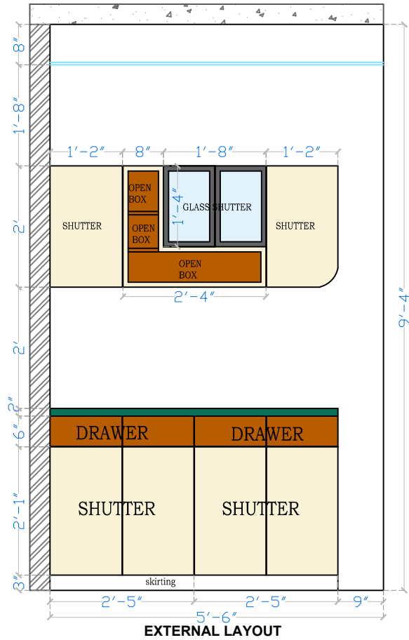
EXTERNAL LAYOUT
