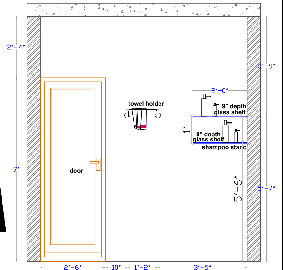
ELEVATION A MASTER ROOM, BATHROOM WORKING DRAWING
