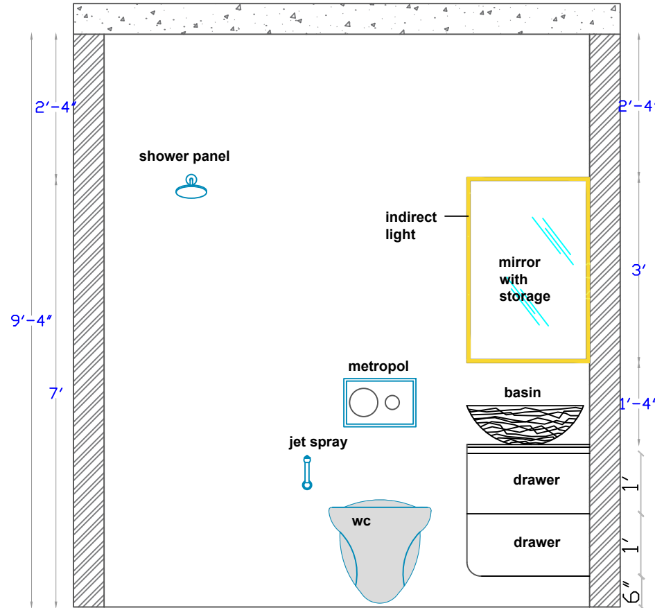
ELEVATION A EXTERNAL LAYOUT
