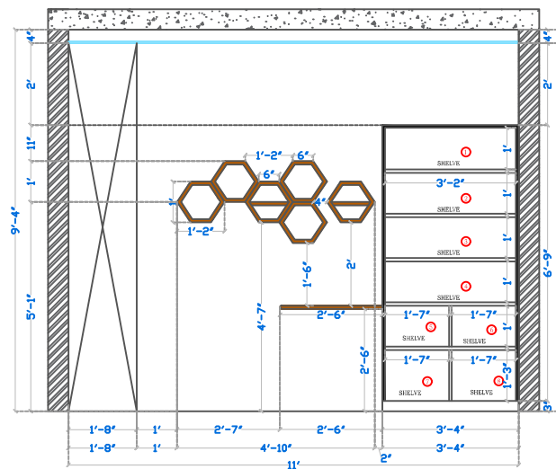
ELEVATION C INTERNAL LAYOUT
