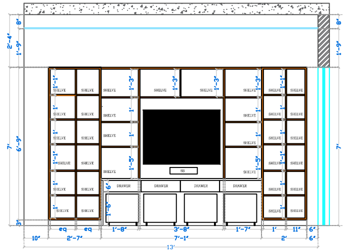
ELEVATION A INTERNAL LAYOUT
