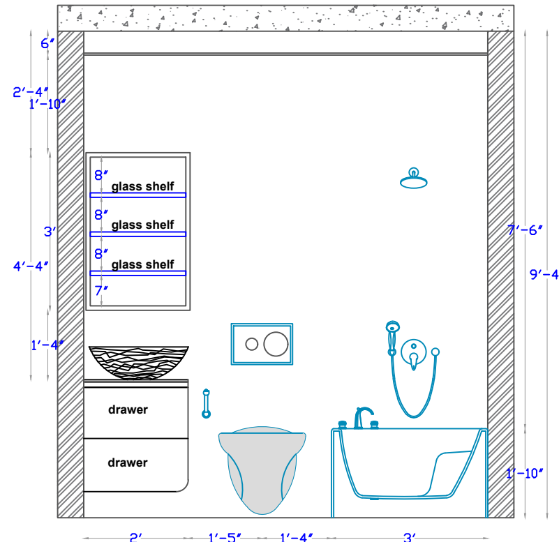
ELEVATION A INTERNAL LAYOUT
